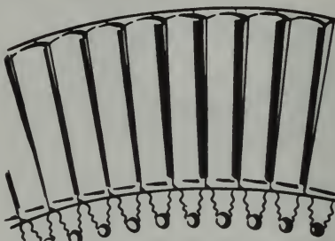
FIGURE 1-54. Riveting method of turbine blade retention.
